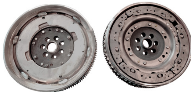
Image 1: Visual comparison of LuK DMF (left) and OE DMF (right)
