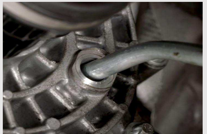
Step 14 Refill the gearbox with oil specified by car manufacturer
