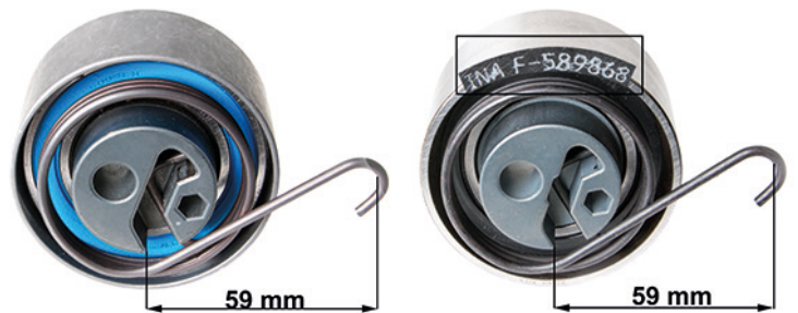
Fig. 2: 531 0819 10 – Old design (left), new design (right)
