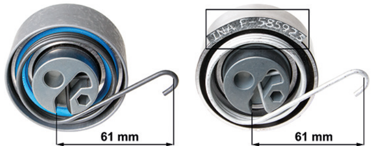
Fig. 1: 531 0535 20 – Old design (left), new design (right)
