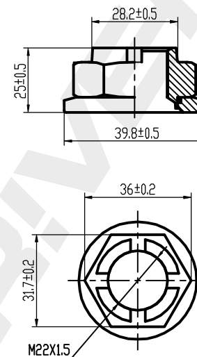
NUT 1PCS The surface is galvanized and the gasket is blackened
