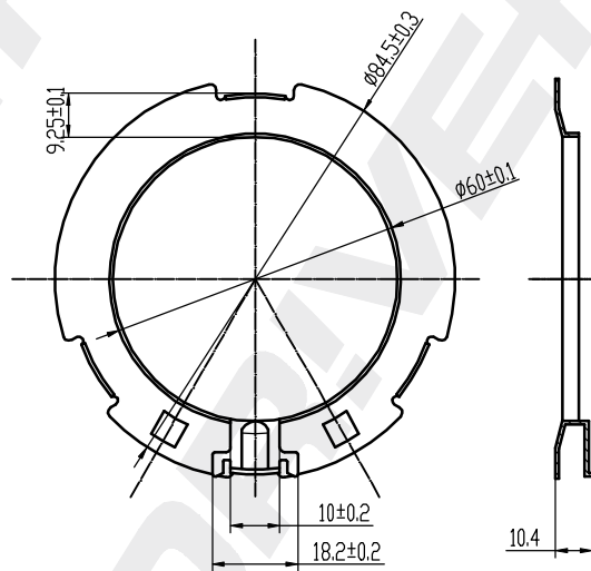
Ring sleeve 1PCS Electroplating
