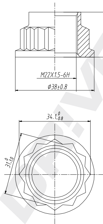
NUT 1pcs Galvanizing
