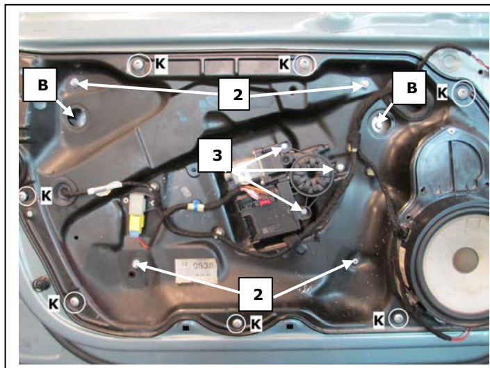
Porta lato sinistro, Portière avant gauche, Left front door, Puerta lado izquierdo, Vorne links Tür, Porta frente esquerda, Sol on kapı, πόρτα εμπρόςα αριστερή
