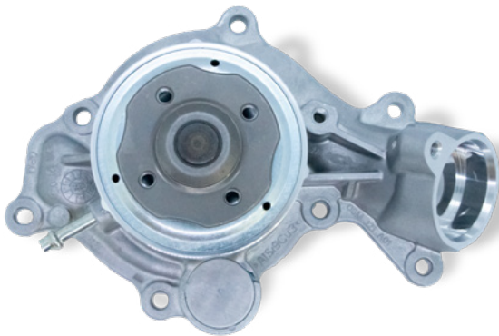
Water pump 7.10942.21.0 with four-hole hub
