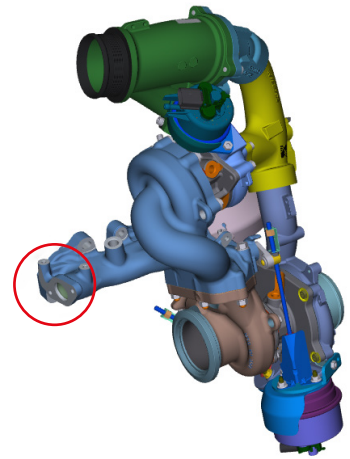
Turbocharger with latest design of EGR flange
