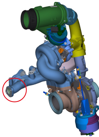
Turbocharger with early design of EGR flange
