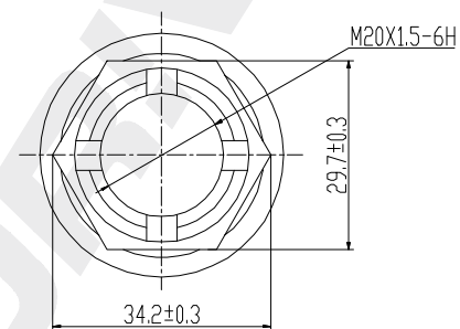
NUT 1pcs Galvanizing
