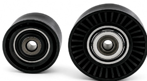
Figure 2: Deflection pulley with new sealing concept (without cap)
